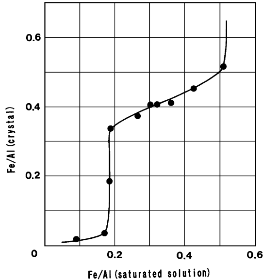
Fig. 1 Compositional relationship between crystal and saturated solution in the system \text{FeSO}_4\text{--Al}_2(\text{SO}_4)_3\text{--H}_2\text{O} , expressed in terms of Fe/Al in molar ratio.
